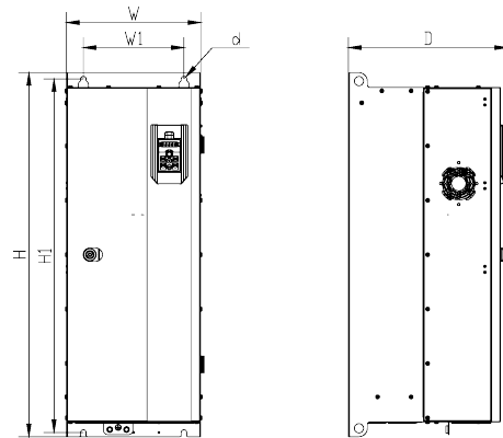
D7-D9 Complete inverter size
